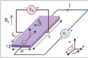
Obr. 9: Geometria Hallovho javu 13
